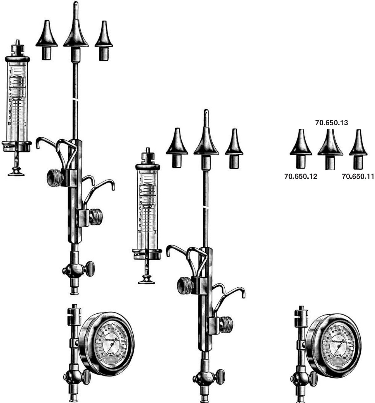
SCHULTZE 70.650.00 compl.
